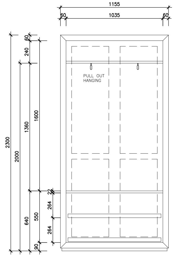
4 - SLIDING SHELVES & HANGING
